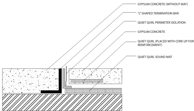
Transition to Gypsum Concrete without mat Quiet Qurl Installation in Hard Surface Areas
