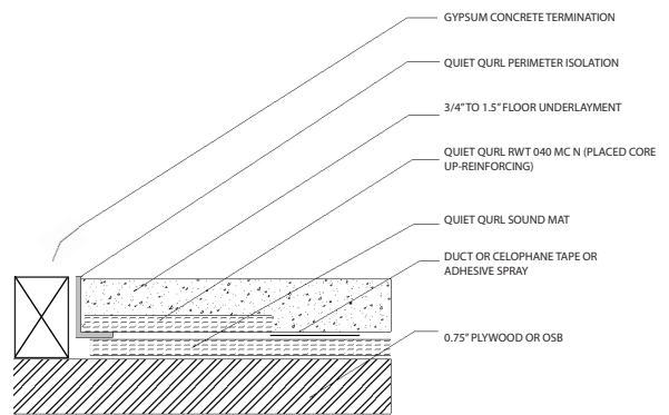
Quiet Qurl Doorway and Floor Transition Detail with Reinforcement
