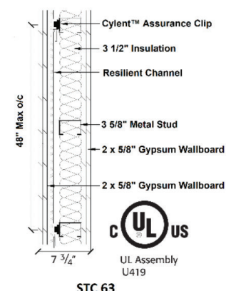
Cylent™ Assurance Clip with 4 Layers
