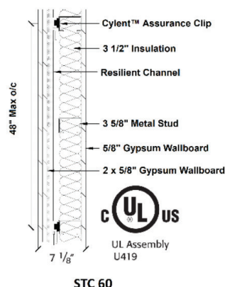
Cylent™ Assurance Clip with 3 Layers
