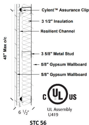
Cylent™ Assurance Clip with 2 layers GWB
